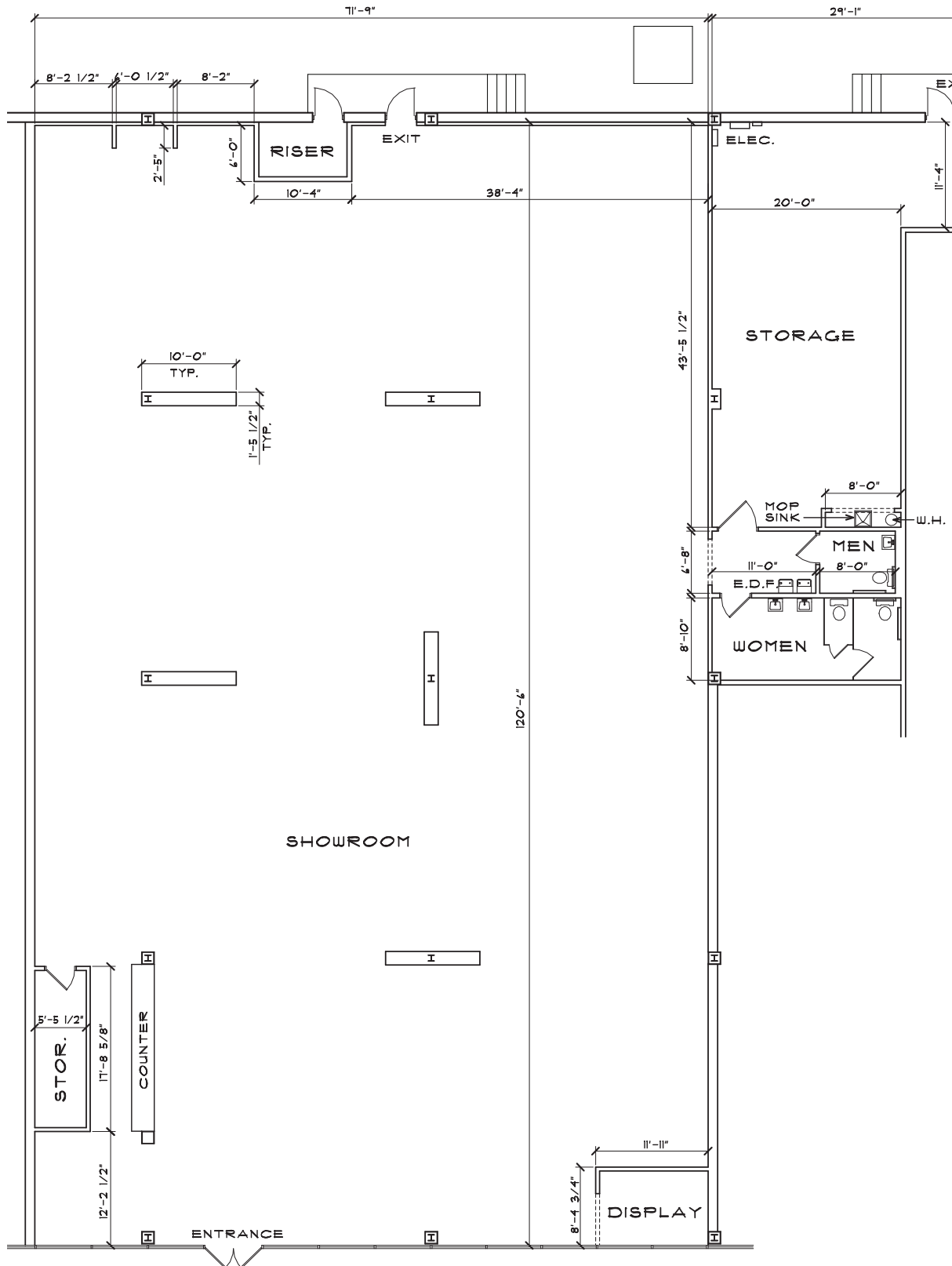
EXISTING FLOOR PLAN 10,088 S.F.
