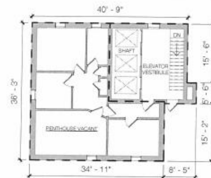
PENTHOUSE FLOOR
