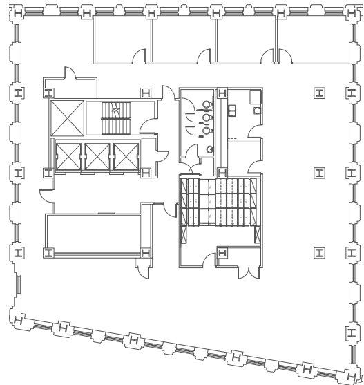
Floor 13 – 5,089 RSF
