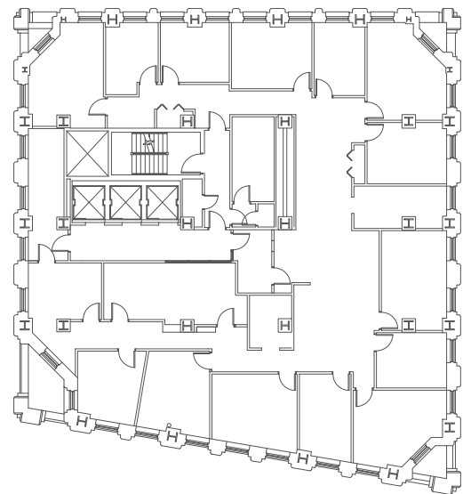
Floor 19 – 5,228 RSF
