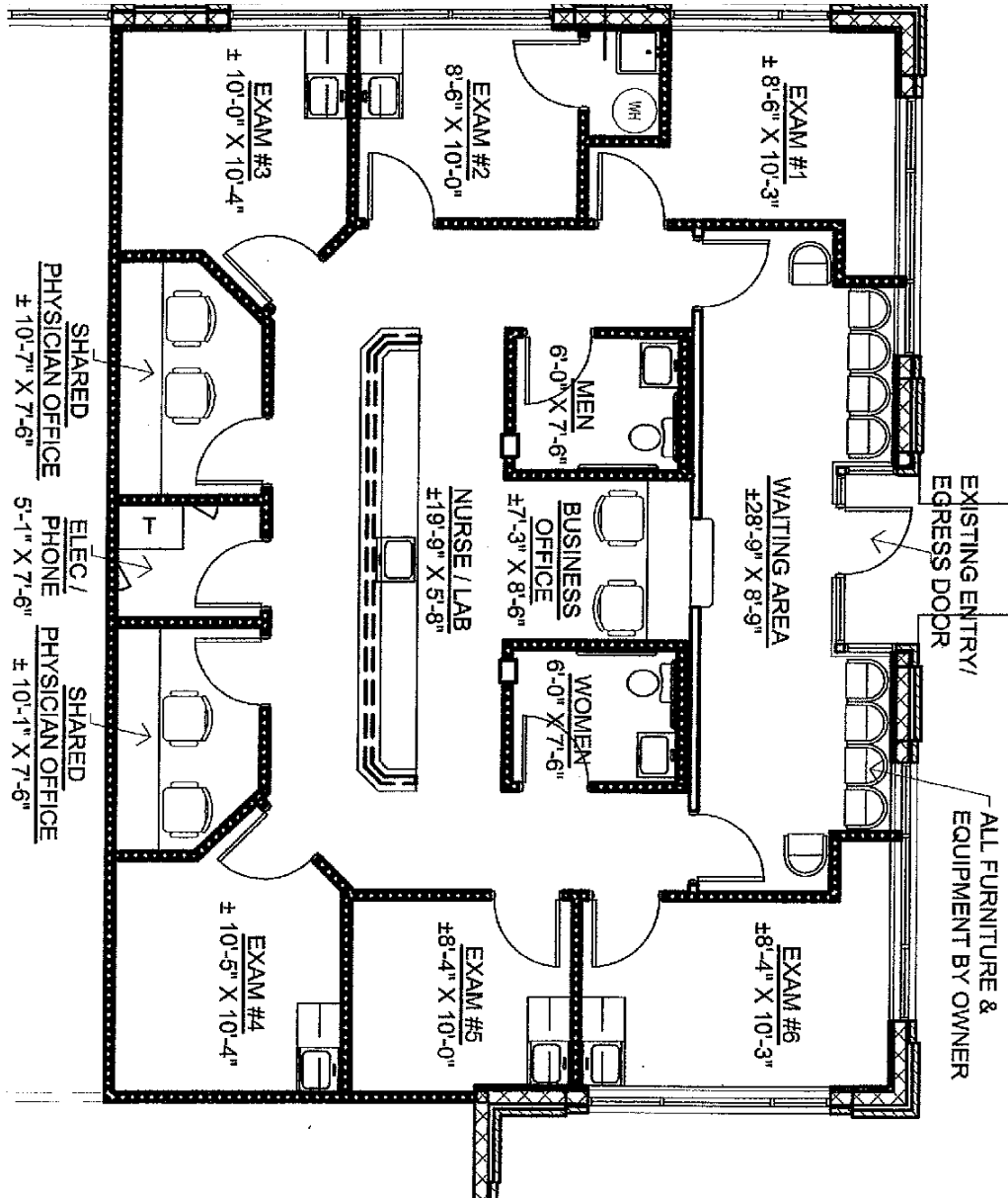
Space Plan #2-1,833 SF
